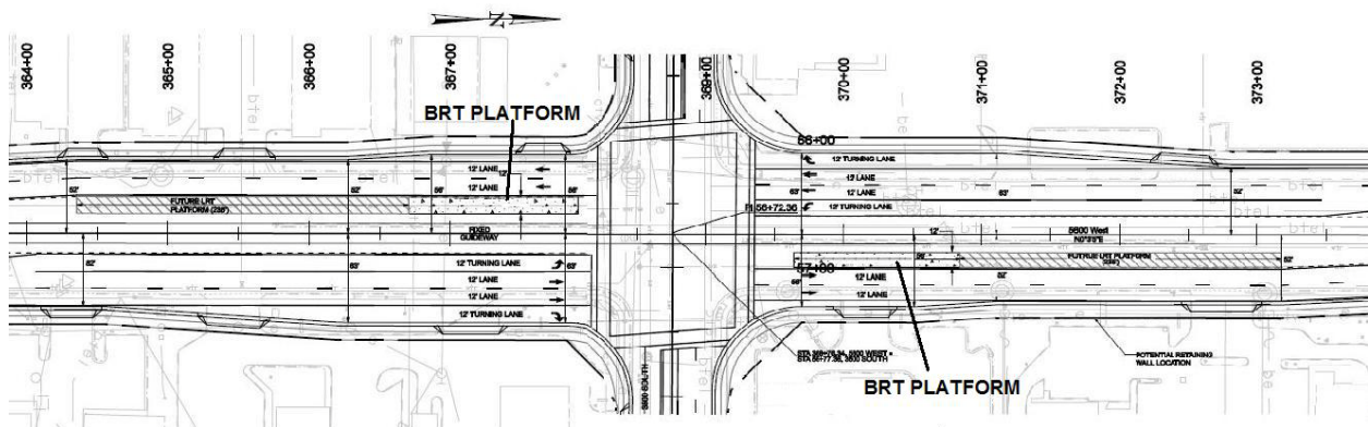
Figure 2.3 Split BRT Stations Design
