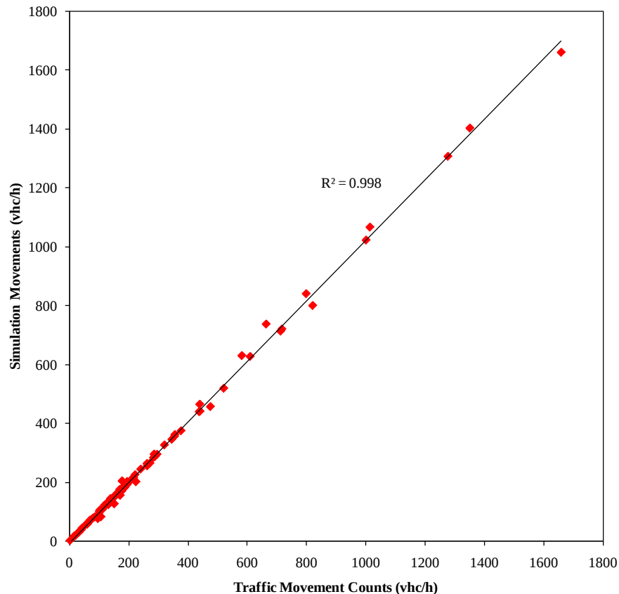
Figure 3.1 Model Calibration Results – Traffic Movement Comparison
