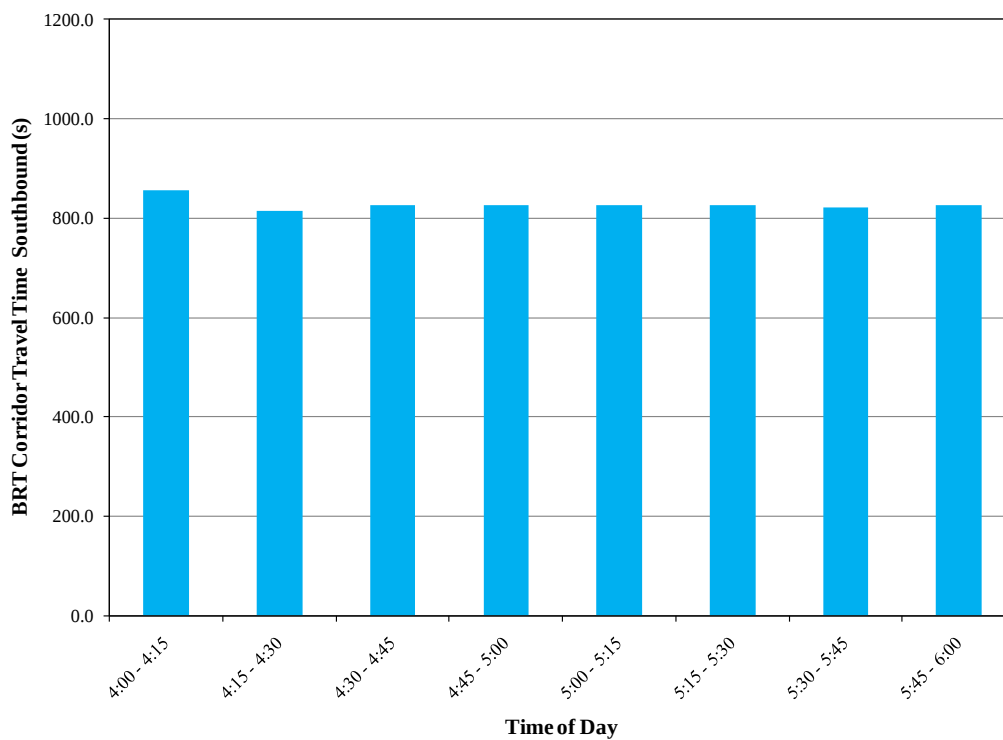
Figure 5.8 15-min BRT Travel Times along the Corridor: 2030 No TSP Transit Scenario a) Southbound; b) Northbound
