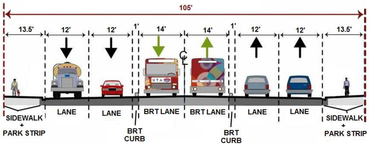
Figure 2.2 Typical Mid-Block Section of 5600 W with 28' BRT Guideway
