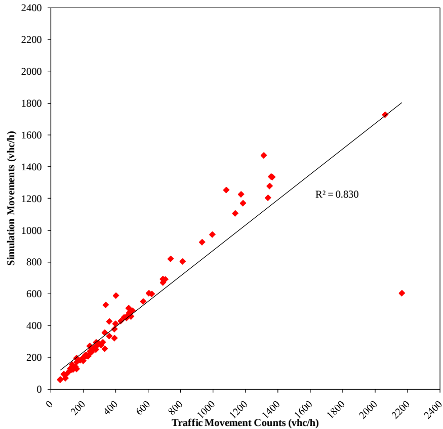
Figure 4.2 2030 Minor Improvements Model Calibration
