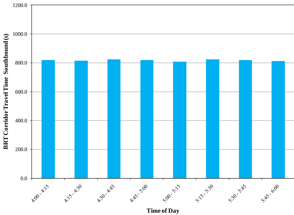
Figure 5.9 15-min BRT Travel Times along the Corridor: 2030 TSP Transit Scenario a) Southbound; b) Northbound
