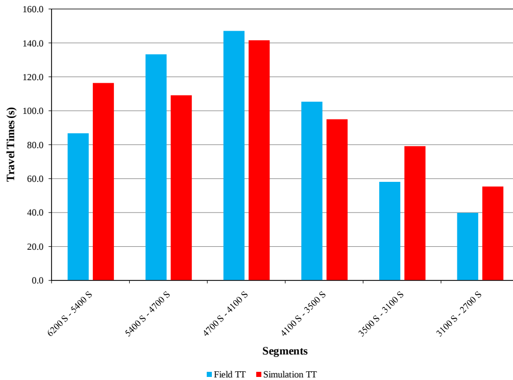
Figure 3.2 Model Validation – Travel Times Comparison a) Southbound; b) Northbound
